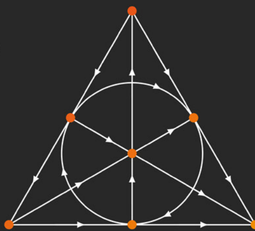
MATROIDS
