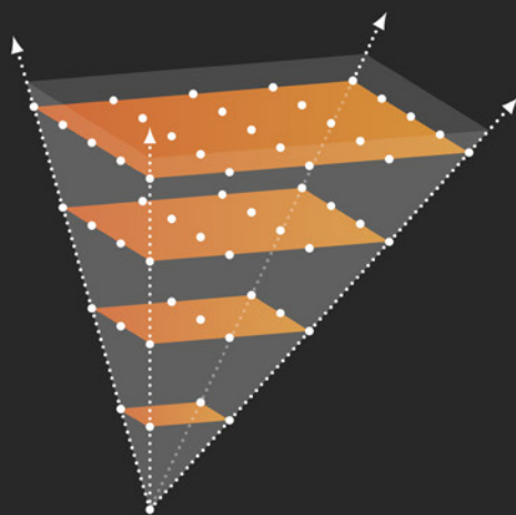
LATTICE POINTS
