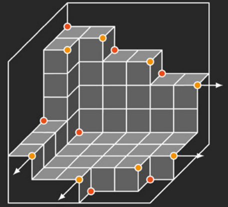
COMMUTATIVE ALGEBRA
