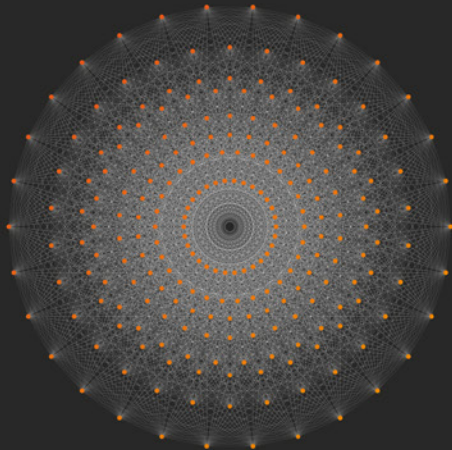
DYNKIN CLASSIFICATION
