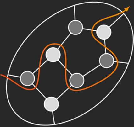
MATHEMATICAL PHYSICS
