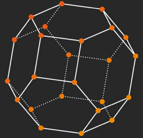
CONVEXITY
