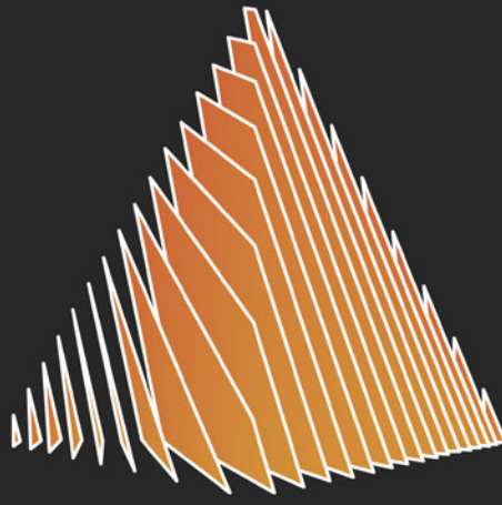
STATISTICS
